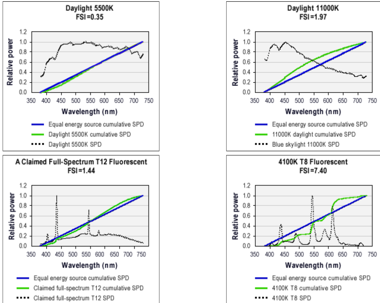
Figure 5. Relative cumulative SPDs for two phases of daylight and several electric light sources.
